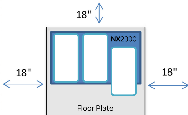
NX2000 machine dimensions w 35.5" x d 23.6" x h 78"
